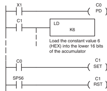
DirectSOFT 5 (optional latch example using SP56)
