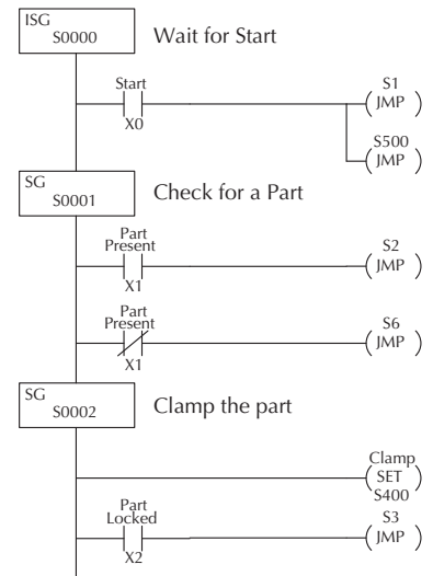
Ladder Representation
